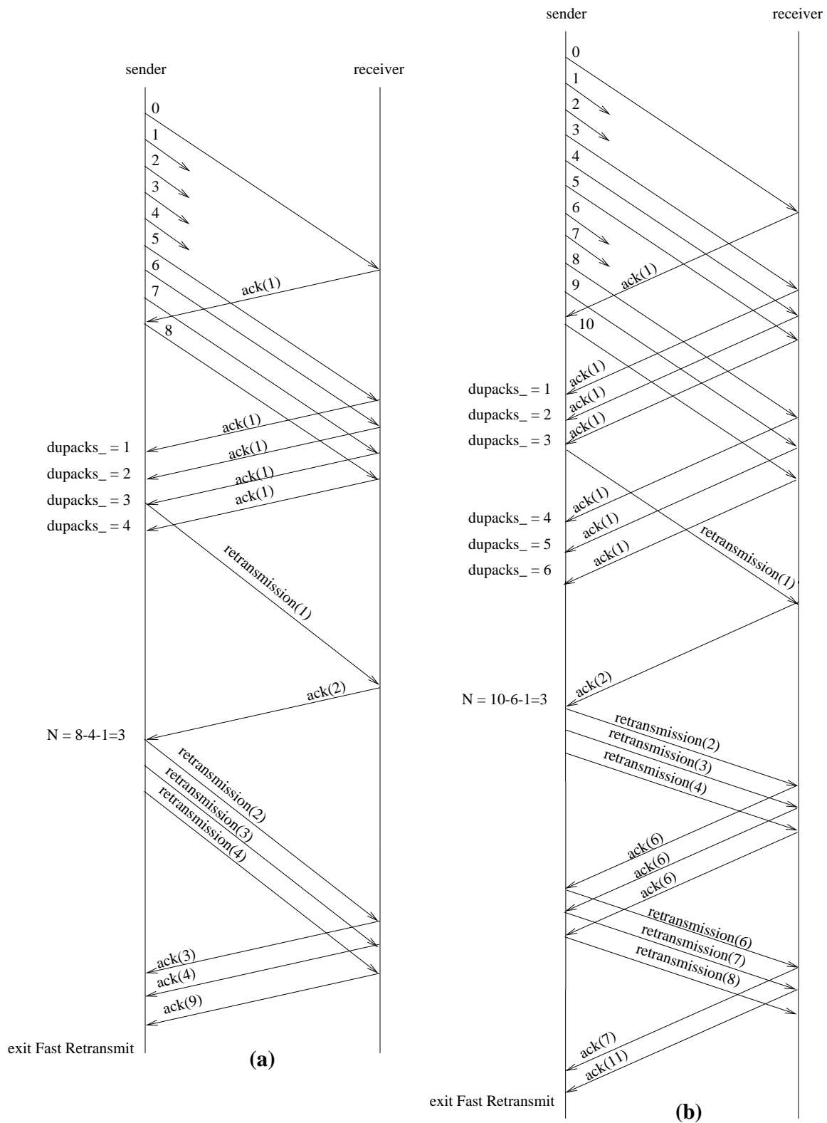
Figure 14: Algorithm execution for one (a) and two (b) holes in the packet sequence.
