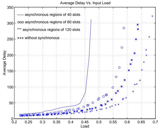
Figure 3: The Performance of the Asynchronous Channel When the HE needs to Ignore Successful Reservations
