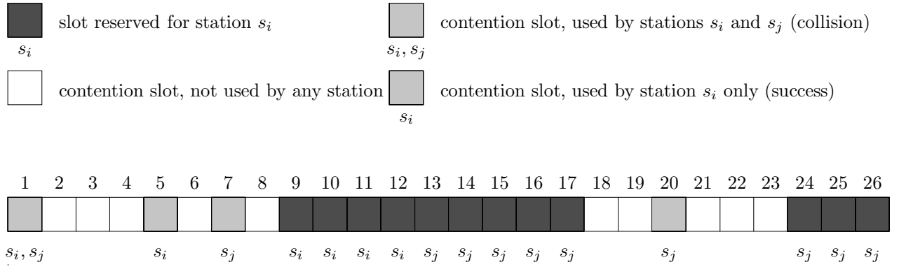
Figure 1: MXL Execution Example
