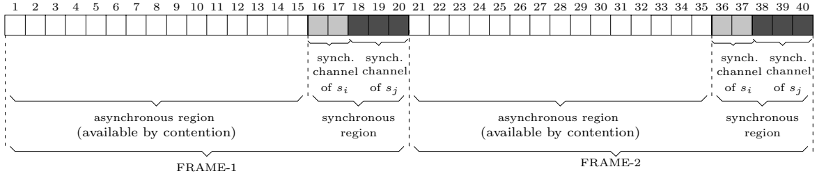
Figure 2: A Naive Approach for Synchronous Traffic Support
