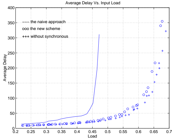
Figure 5: The Performance of the Asynchronous Channel When the New Scheme is Employed
